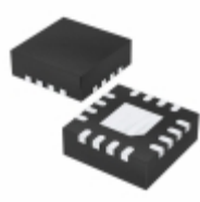
PIC16F630-I/ML Microchip Technology IC MCU 8BIT 1.75KB FLASH 16QFN
