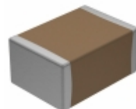
VJ1812Y104KXCAT Vishay Vitramon CAP CER 0.1UF 200V X7R 1812
