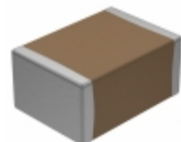
VJ1812Y104KXBAT Electro-Films (EFI) / Vishay CAP CER 0.1UF 100V X7R 1812
