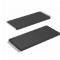
AT27C010-55TC Microchip Technology IC OTP 1MBIT 55NS 32TSOP
