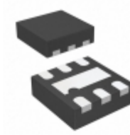
MIC5338-MGYMT-TR Microchip Technology IC REG LDO 2.8V/1.8V 0.3A 6TMLF
