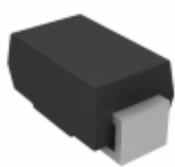
CSA2G-E3/I Vishay Semiconductor Diodes Division DIODE GPP 2A 400V DO-214AC SMA
