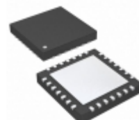
PIC16LF648A-I/ML Microchip Technology IC MCU 8BIT 7KB FLASH 28QFN
