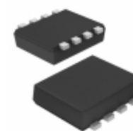
QS8J4TR Rohm Semiconductor MOSFET 2P-CH 30V 4A TSMT8
