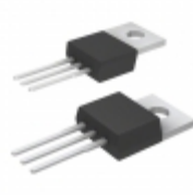
IXFP10N80P IXYS MOSFET N-CH 800V 10A TO-220
