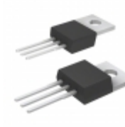
IXFP110N15T2 IXYS MOSFET N-CH 150V 110A TO-220
