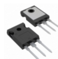
IRGP50B60PD1-EP Infineon Technologies IGBT 600V 75A 390W TO247AD
