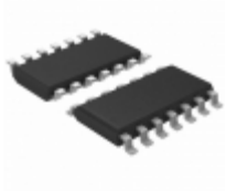
MAX4078ESD+T Maxim Integrated IC OPAMP GP 230KHZ RRO 14SOIC
