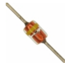
MTZJT-7718B Rohm Semiconductor DIODE ZENER 18V 500MW MSD
