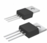
DHG20C1200PB IXYS DIODE ARRAY GP 1200V 10A TO220AB
