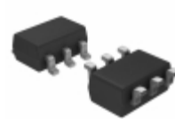
MCP4716A1T-E/CH Microchip Technology IC DAC 10BIT NV EEP I2C SOT-23-6
