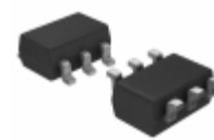
MCP4725A3T-E/CH Microchip Technology IC DAC 12BIT EE W/I2C SOT23-6
