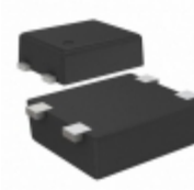
S-80833CLPF-B6STFU SII Semiconductor Corporation IC VOLT DETECTOR 3.3V SNT-4A
