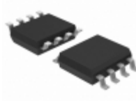
X9313US Intersil IC DIGITAL POT 50K 32TP 8SOIC
