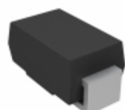
SSA24HE3/5AT Vishay Semiconductor Diodes Division DIODE SCHOTTKY 40V 2A DO214AC
