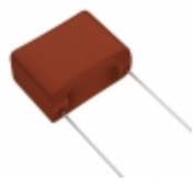
ECW-F2W475JA Panasonic Electronic Components CAP FILM 4.7UF 5% 450VDC RADIAL
