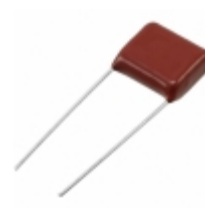
ECQ-E2125KF3 Panasonic Electronic Components CAP FILM 1.2UF 10% 250VDC RADIAL
