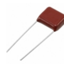
ECQ-E2125KFB Panasonic Electronic Components CAP FILM 1.2UF 10% 250VDC RADIAL
