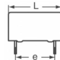
B32676G4106J000 EPCOS CAP FILM 10UF 5% 450VDC RADIAL
