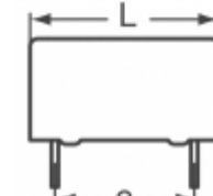
B32676G4106J EPCOS (TDK) CAP FILM 10UF 5% 450VDC RADIAL
