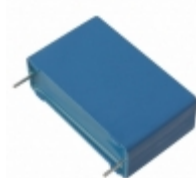
B32676G4156K000 EPCOS CAP FILM 15UF 10% 450VDC RADIAL
