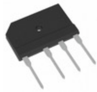
TS25P01G D2G TSC (Taiwan Semiconductor) BRIDGE RECT 1PHASE 50V 25A TS-6P
