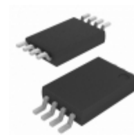
IRF7706TRPBF International Rectifier (Infineon Technologies) MOSFET P-CH 30V 7A 8-TSSOP
