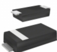
CZRA4746-HF Comchip Technology DIODE ZENER 18V 1W DO214AC
