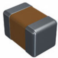
CDR31BX471BKMSAP Electro-Films (EFI) / Vishay CAP CER 470PF 100V BX 0805
