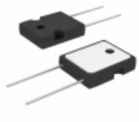
VS-E4PU6006LHN3 Electro-Films (EFI) / Vishay DIODE GEN PURP 600V 60A TO247AD
