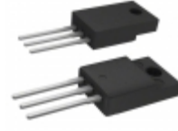
BYVF32-100-E3/45 Electro-Films (EFI) / Vishay DIODE ARRAY GP 100V 18A ITO220AB
