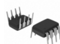
LT1673CN8#PBF ADI (Analog Devices, Inc.) IC OPAMP GP 12KHZ RRO 8DIP
