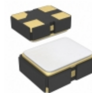
SG-8003CE-PCL EPSON OSC PROG CMOS 3.3V EN/DS 50PPM
