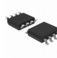
AT34C02D-SSHM-T Microchip Technology IC EEPROM 2KBIT 1MHZ 8SOIC
