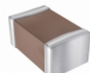
08051C102KAT2M AVX Corporation CAP CER 1000PF 100V X7R 0805
