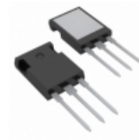
IXGR6N170A IXYS IGBT 1700V 5.5A 50W ISOPLUS247
