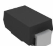
TPSMA43AHE3/61T Vishay Semiconductor Diodes Division TVS DIODE 36.8VWM 59.3VC SMA
