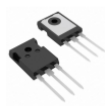
IXXH75N60C3 IXYS IGBT 600V 150A 750W TO247
