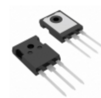
IXXH50N60C3 IXYS IGBT 600V 100A 600W TO247AD
