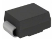
ATV06B221JB-HF Comchip Technology TVS DIODE 220VWM 356VC DO214AA
