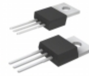
DPG30C400PB IXYS DIODE ARRAY GP 400V 15A TO220AB
