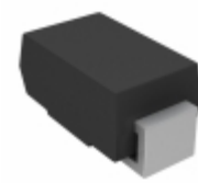
SMAJ13CA-E3/5A Electro-Films (EFI) / Vishay TVS DIODE 13V 21.5V DO214AC
