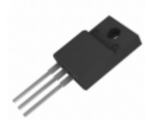
FQPF8N60CT Fairchild/ON Semiconductor MOSFET N-CH 600V 7.5A TO-220F
