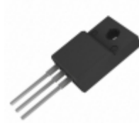
FQPF8N80C Fairchild/ON Semiconductor MOSFET N-CH 800V 8A TO-220F
