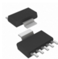
MCP1825T-3002E/DC Microchip Technology IC REG LDO 3V 0.5A SOT223-5
