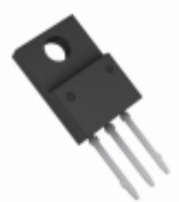
BA78M18CP-E2 Rohm Semiconductor IC REG LDO 18V 0.5A TO220CP-3
