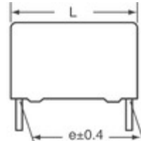
B32923C3394K EPCOS (TDK) CAP FILM 0.39UF 10% 305VAC RAD
