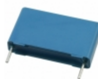
B32923C3334M289 EPCOS (TDK) CAP FILM 0.33UF 20% 305VAC RAD
