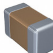
C0603C102K5RAC7411 KEMET CAP CER SMD 0603 1000PF 10% X7R
