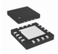
ADG5408TCPZ-EP Analog Devices Inc. IC MUX 8:1 14 OHM 16LFCSP
