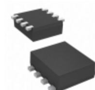
FC8V33030L Panasonic Electronic Components MOSFET 2N-CH 33V 6.5A WMINI8
