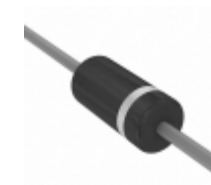
P6KE13A-E3/54 Vishay Semiconductor Diodes Division TVS DIODE 11.1VWM 18.2VC DO204AC
