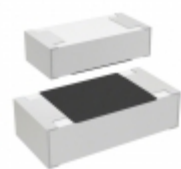
CR0603-JW-914ELF Bourns Inc. RES SMD 910K OHM 5% 1/10W 0603
