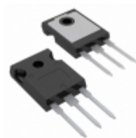
IRGP4660D-EPBF Infineon Technologies IGBT 600V 100A 330W TO247AD
