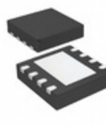
MCP4542T-103E/MF Microchip Technology IC DGTL POT 10K 129TAPS 8-DFN
