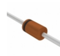
1N4742A,133 Nexperia USA Inc. DIODE ZENER 12V 1W DO41
