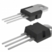
MIC39150-2.5BT Microchip Technology IC REG LDO 2.5V 1.5A TO220-3
