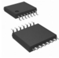
74VHC00MTC AMI Semiconductor / ON Semiconductor IC GATE NAND 4CH 2-INP 14TSSOP
