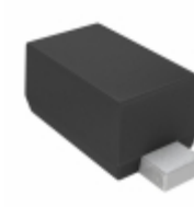
VDZT2R3.0B Rohm Semiconductor DIODE ZENER 3V 100MW VMD2
