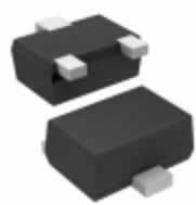
VDZT2R2.2B Rohm Semiconductor DIODE ZENER 2.2V 100MW VMD3
