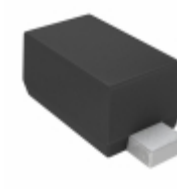
VDZT2R20B Rohm Semiconductor DIODE ZENER 20V 100MW VMD2
